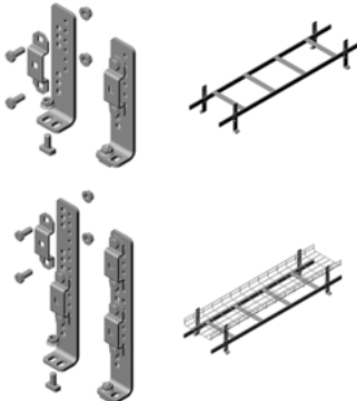
Cabinet Mounting
